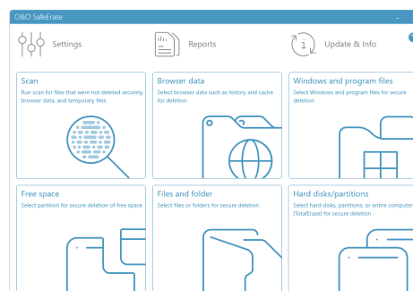
Start page
