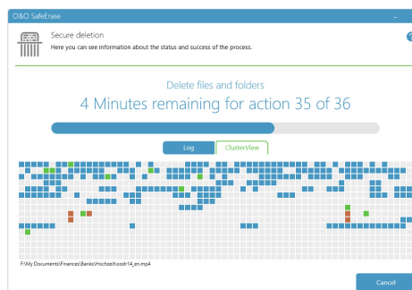
ClusterView
