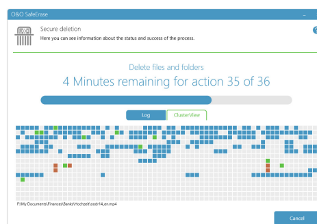
ClusterView
