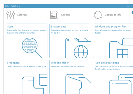
Start page
