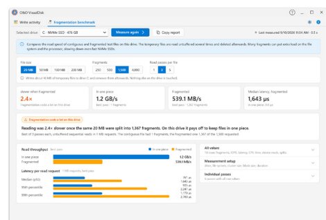
O&O VisualDisk - Fragmentation benchmark
