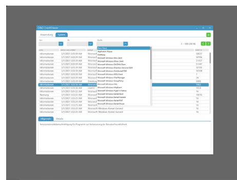
O&O EventViewer
